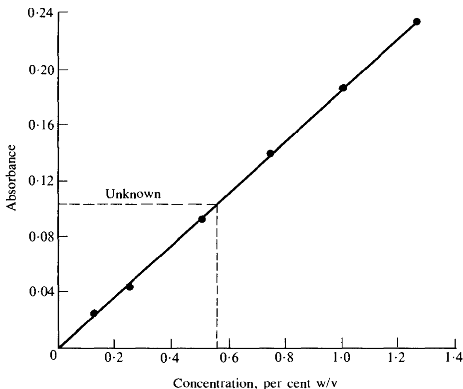
Fig. 19.9 Calibration graph for antioxidant determination.
