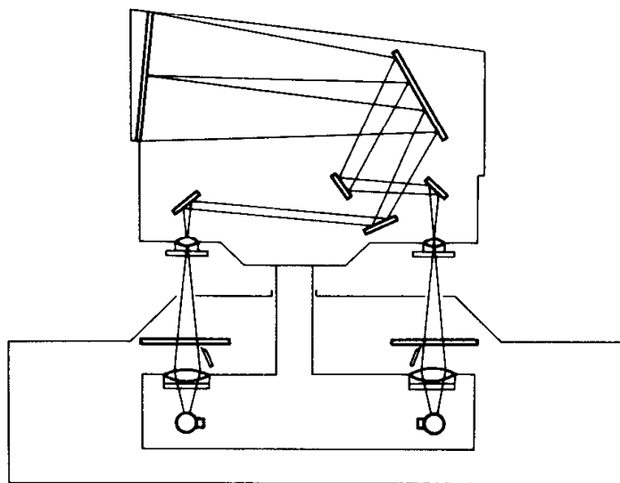
Fig. 20.5 The Rank Hilger L150 projection comparator.
