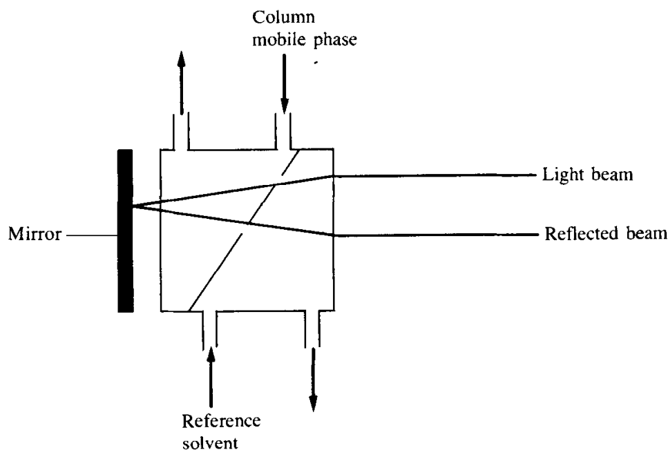
Fig. 8.4 Refractive index detector.
