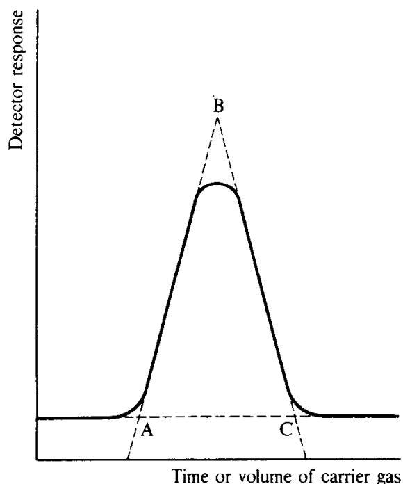
Fig. 9.3 Measurement of peak area by triangulation.
