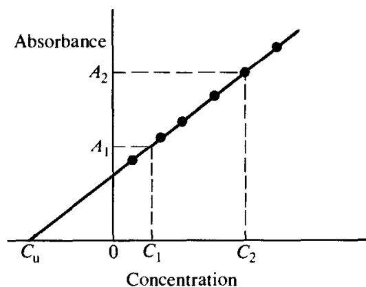
Fig. 19.10 Calibration plot for standard addition procedure.
