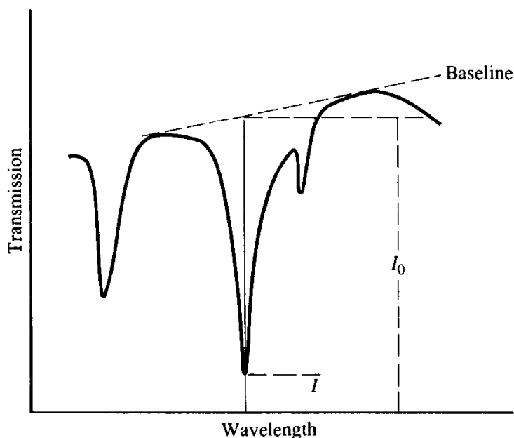
Fig. 19.8 Tangent baseline measurement.
