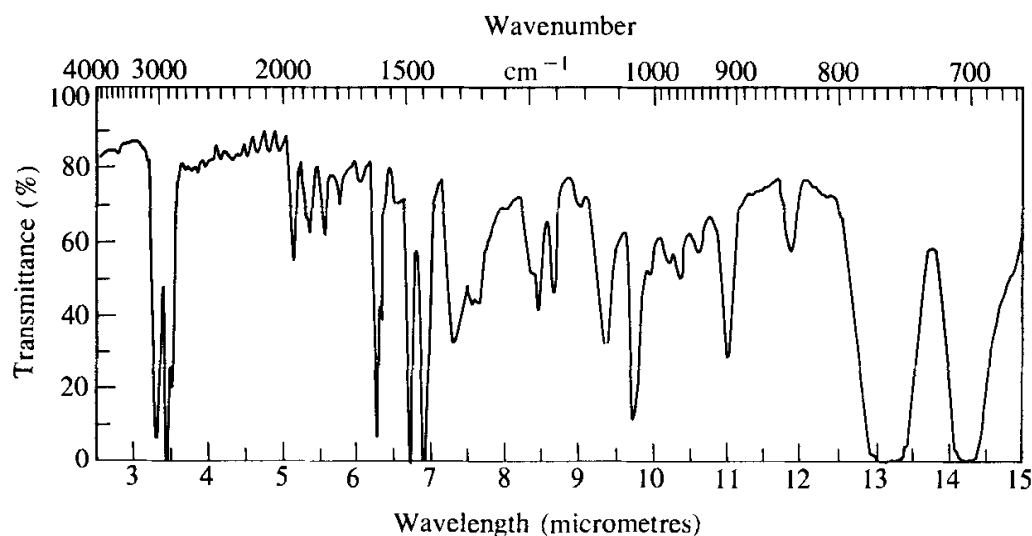
Fig. 19.1 The infrared spectrum of polystyrene.
