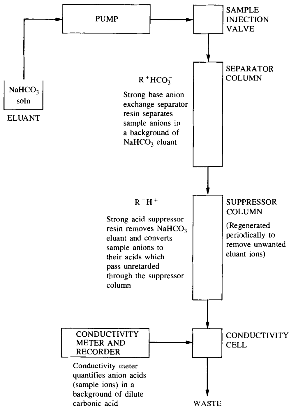
Fig. 7.3 Ion chromatography flow scheme (anion analysis).
