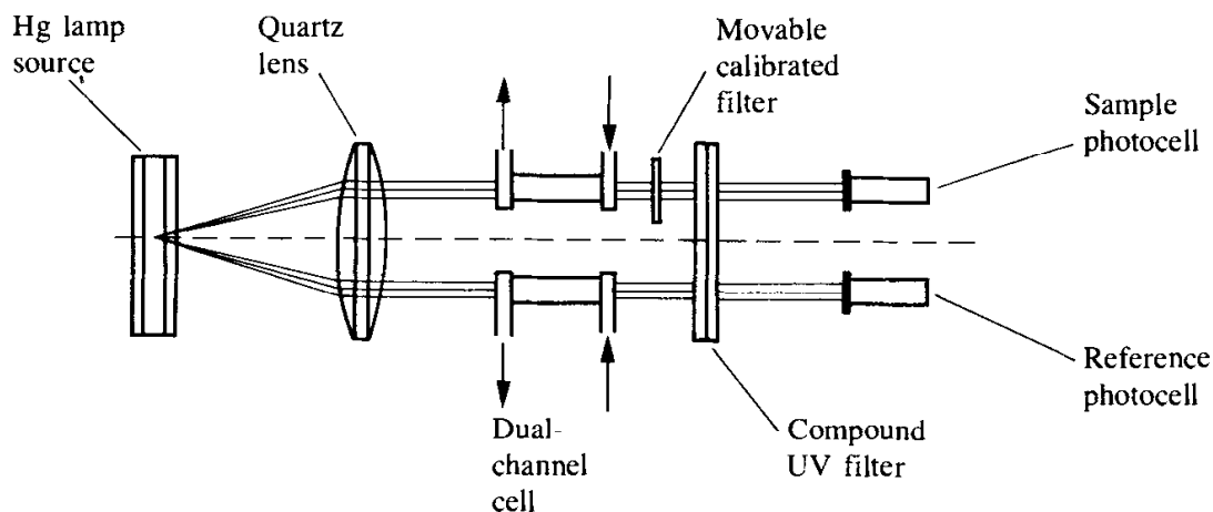
Fig. 8.5 Block diagram of a double-beam UV detector.
