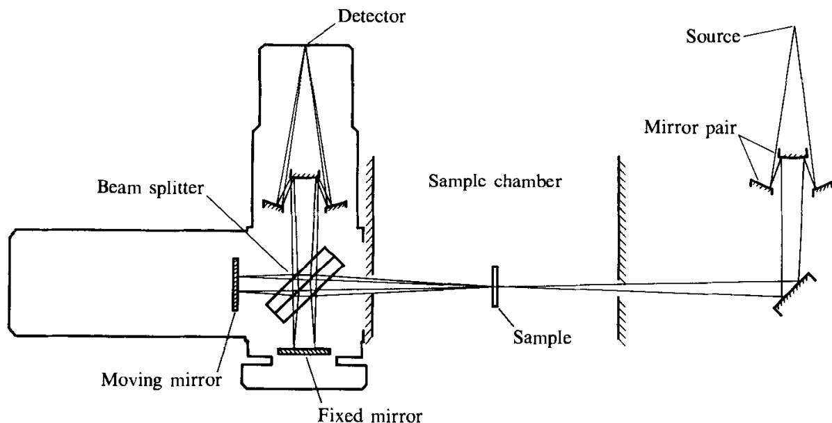
Fig. 19.3 Layout of a Fourier-transform infrared spectrometer. Reproduced by permission of Lloyd Instruments PLC, Warsash, Southampton SO3 6HP.
