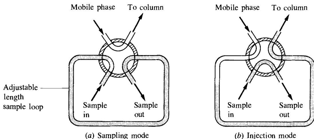
Fig. 8.3 Operation of a sample loop.
